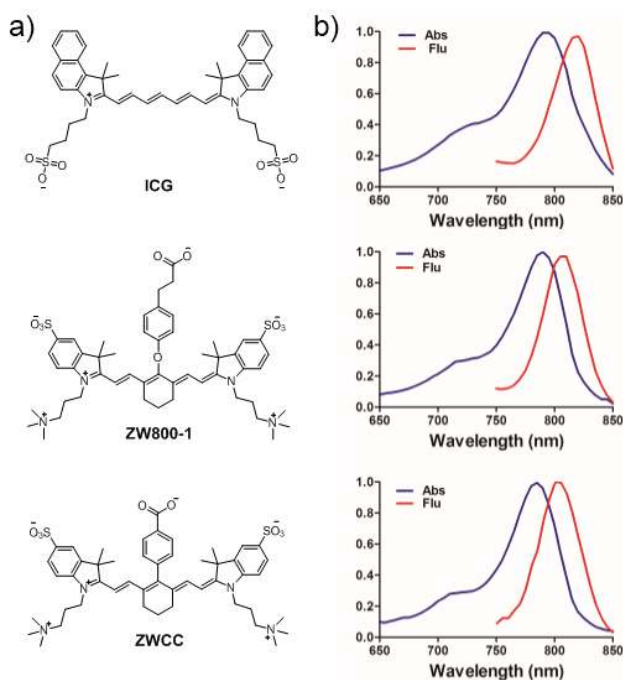
Fig. 1 (a) Chemical structures of ICG , ZW800-1 and ZWCC ; (b) Normalized absorbance and fluorescence spectra of each fluorophore (5 \mu\text{M} in DMSO, \lambda_{\text{ex}} = 730 \text{ nm} ).
