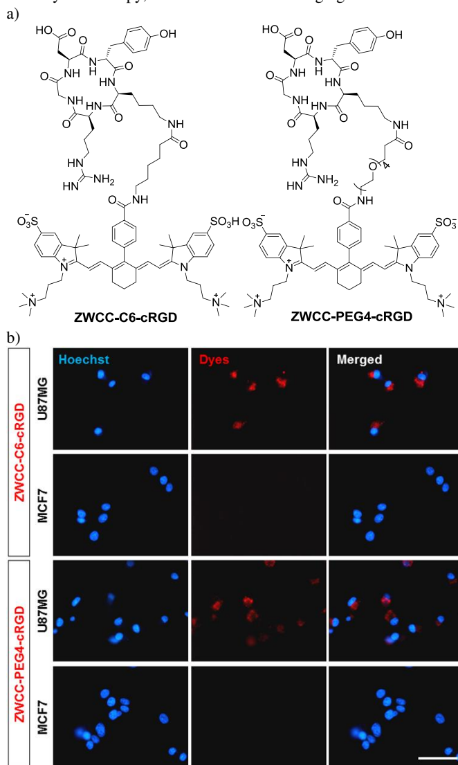
Fig. 3 Structures (a) and fluorescence cell imaging of ZWCC -linker-cRGD (b). Red colour is from ZWCC compounds (middle panels) and blue colour is from Hoechst stain (left panels) for nuclei visualization. Right panels show merged images of the two. Images were captured by 40x objective. Scale bar is 50 \mu\text{m} .
