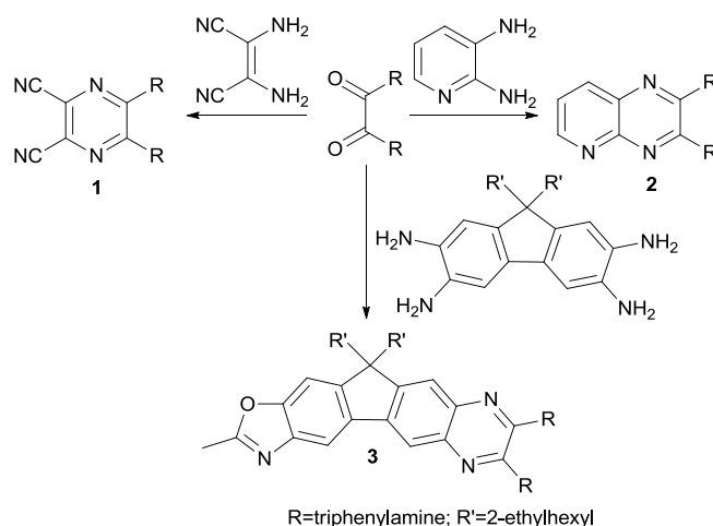
80 Scheme 1 Synthesis route for compounds 1-3 . Conditions: anhydrous acetic acid, Ar 2 , 2-iodoxybenzoic acid, 120°C, 24 h.
