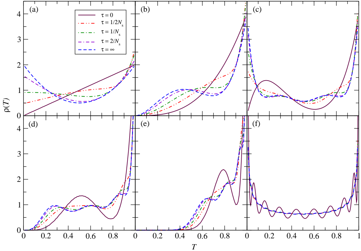
Figure 2. The density of transmission eigenvalues \rho(T) = \mathcal{R}_1(T)/N for SE-UE crossover at various \tau for (a) N_1 = 2, N_2 = 2 , (b) N_1 = 2, N_2 = 4 , (c) N_1 = 4, N_2 = 4 , (d) N_1 = 4, N_2 = 8 , (e) N_1 = 4, N_2 = 20 and (f) N_1 = 20, N_2 = 20 .
