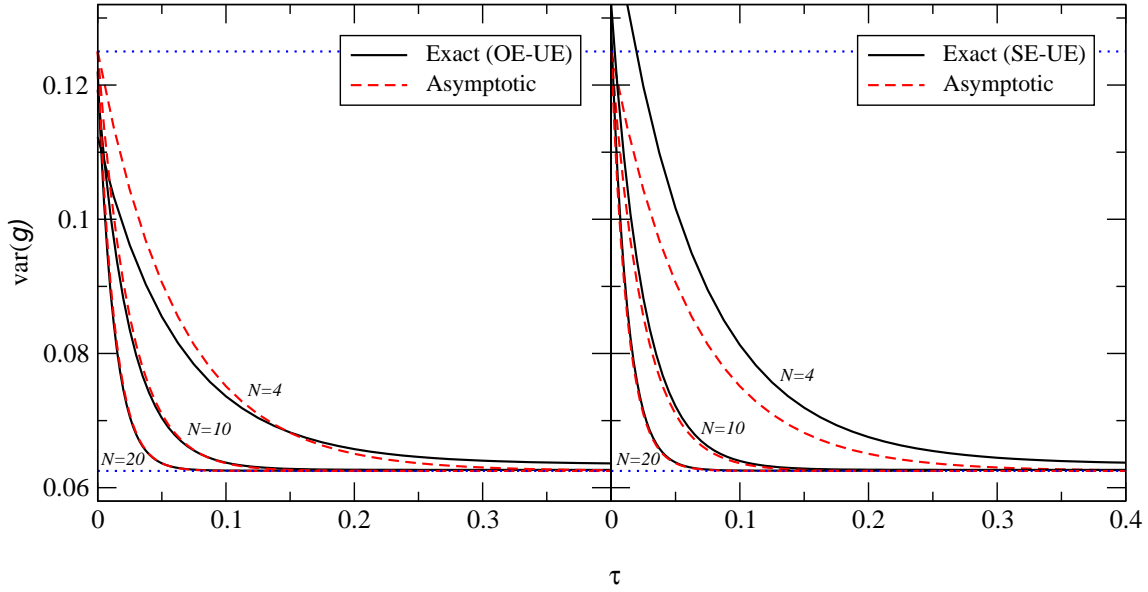
Figure 3. The variance of conductance as a function of \tau for various N (= N_1 = N_2) for the two transitions. The dotted horizontal lines represent the universal values 1/8 and 1/16 .
