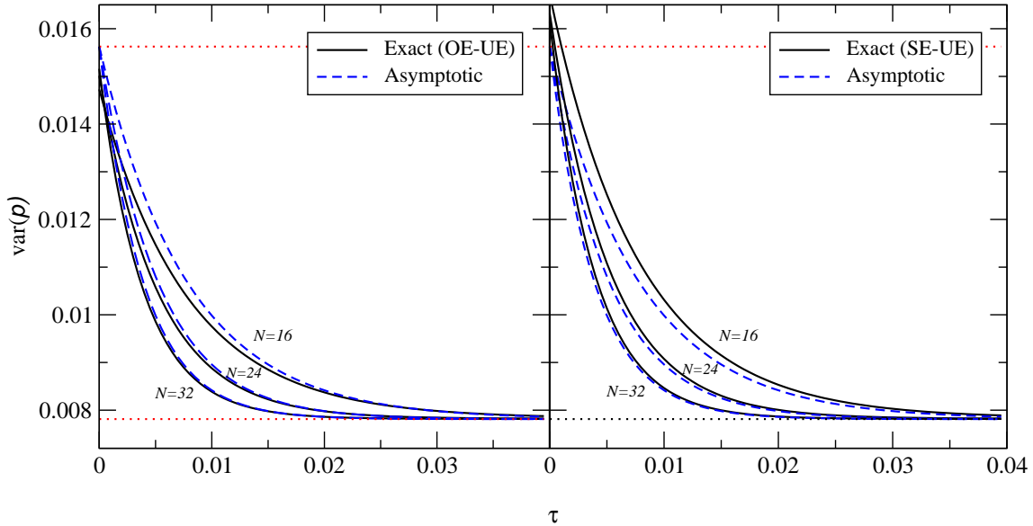
Figure 4. The variance of shot-noise power as a function of \tau for various N (= N_1 = N_2) for the two transitions. The dotted horizontal lines represent the universal values 1/64 and 1/128 .
