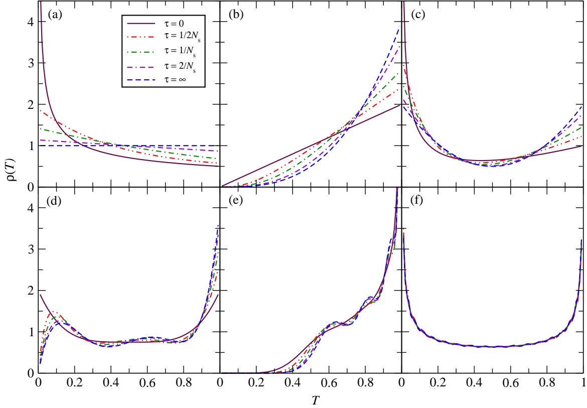
Figure 1. The density of transmission eigenvalues \rho(T) = \mathcal{R}_1(T)/N for OE-UE crossover for several values of \tau for (a) N_1 = 1, N_2 = 1 , (b) N_1 = 1, N_2 = 4 , (c) N_1 = 2, N_2 = 2 , (d) N_1 = 3, N_2 = 4 , (e) N_1 = 4, N_2 = 20 , (f) N_1 = 20, N_2 = 20 .
