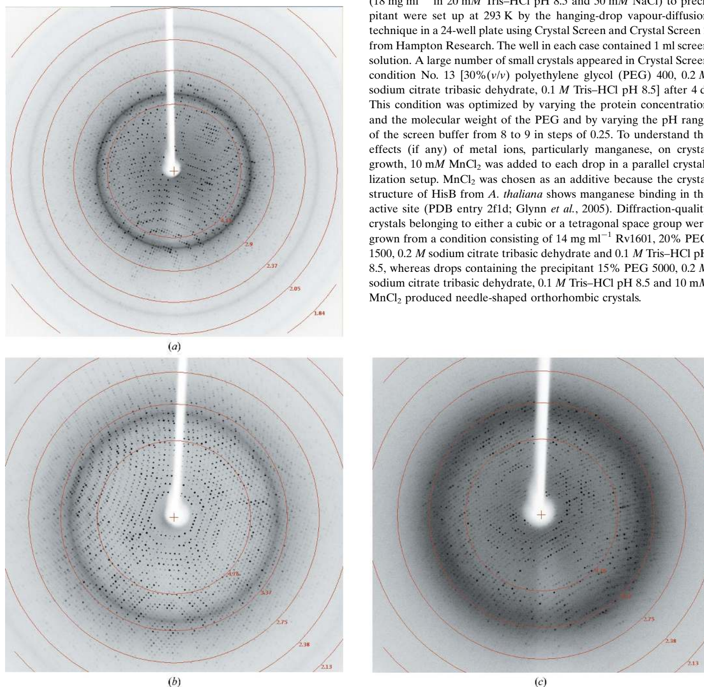
Figure 3 Representative diffraction images of (a) cubic, (b) tetragonal and (c) orthorhombic crystals. The resolution rings are shown by the red concentric circles.
