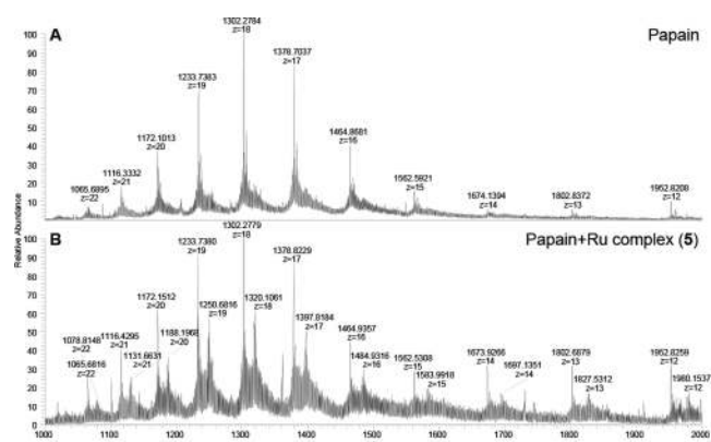
Figure 6. ESI-HRMS mass spectra of (A) papain and (B) bioconjugate 5 , both at 2.15 \mu\text{M} in water/acetonitrile/formic acid (49:50:1, v/v/v).
