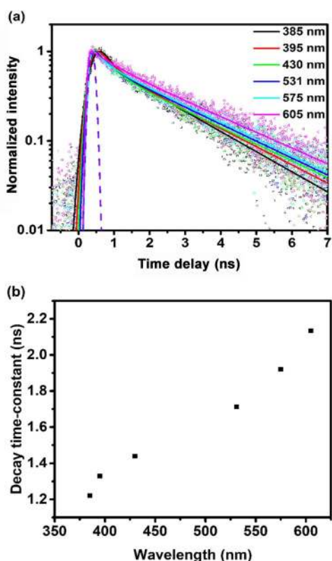
Figure 6. (a) (CyBMA)PbBr 4 time-resolved PL decays. Excitation wavelength is 340 nm at 50 \mu\text{J cm}^{-2} fluence and the emission was collected for different emission wavelengths at 298 K. The data were fitted with a stretched exponential equation: I(t) = I_0 \times \exp[-(t/\tau)^\beta] , \tau is the characteristic decay time and \beta is stretching exponent. (b) Decay-times vs. emission wavelengths.
