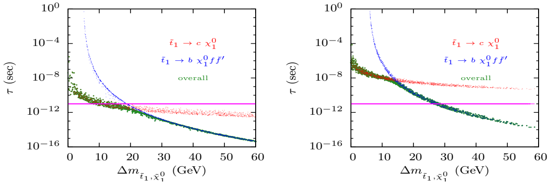
Figure 9. Decay life-time of \tilde{t}_1 (at rest) if only the two-body c\tilde{\chi}_1^0 mode (in red) or only the four-body b\bar{f}\bar{f}'\tilde{\chi}_1^0 mode (in blue) were possible as functions of the mass-split ( \Delta m_{\tilde{t}_1, \tilde{\chi}_1^0} ) between \tilde{t}_1 and \tilde{\chi}_1^0 . Points in green indicate the values of the actual lifetime of \tilde{t}_1 (at rest) and result from summing up its decay widths in the two modes. The left plot is for the case of bino-dominated LSP while the right one stands for the case of the singlino-dominated LSP. The scattered points are obtained by scanning over the NMSSM parameter space. See text for details.
