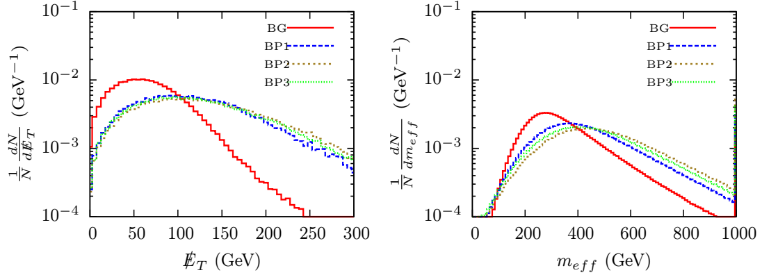
Figure 12. E_T distributions (left) and m_{\text{eff}} distributions (right) for the SM background (in red) and for the signal in the inclusive multilepton final state for the three benchmark points (in blue, brown and green, respectively) and for LHC-13.
