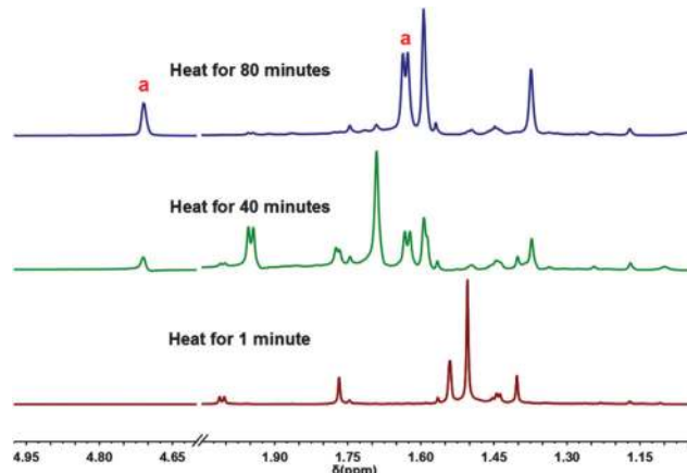
Fig. 2 1 H NMR spectrum of the reaction of P 4 ( \mu -N t Bu) 6 ( 1 ) with elemental Se in a sealed NMR tube under reflux in toluene- d 8 .
