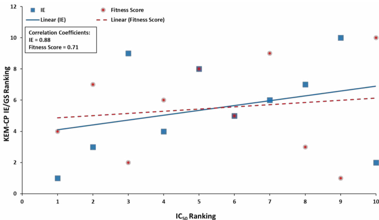
Figure 6. Plot showing IC 50 ranking distribution with the KEM-CP IE and GoldScore Fitness score rankings for the best predicted poses (data from Table S28).
