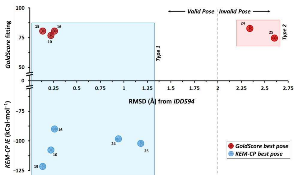
Figure 2. Distribution of RMSD (Å) vs. fitting score from GoldScore and vs. KEM-CP based average IE (Tables 2 and 3) of hAR ligands.
