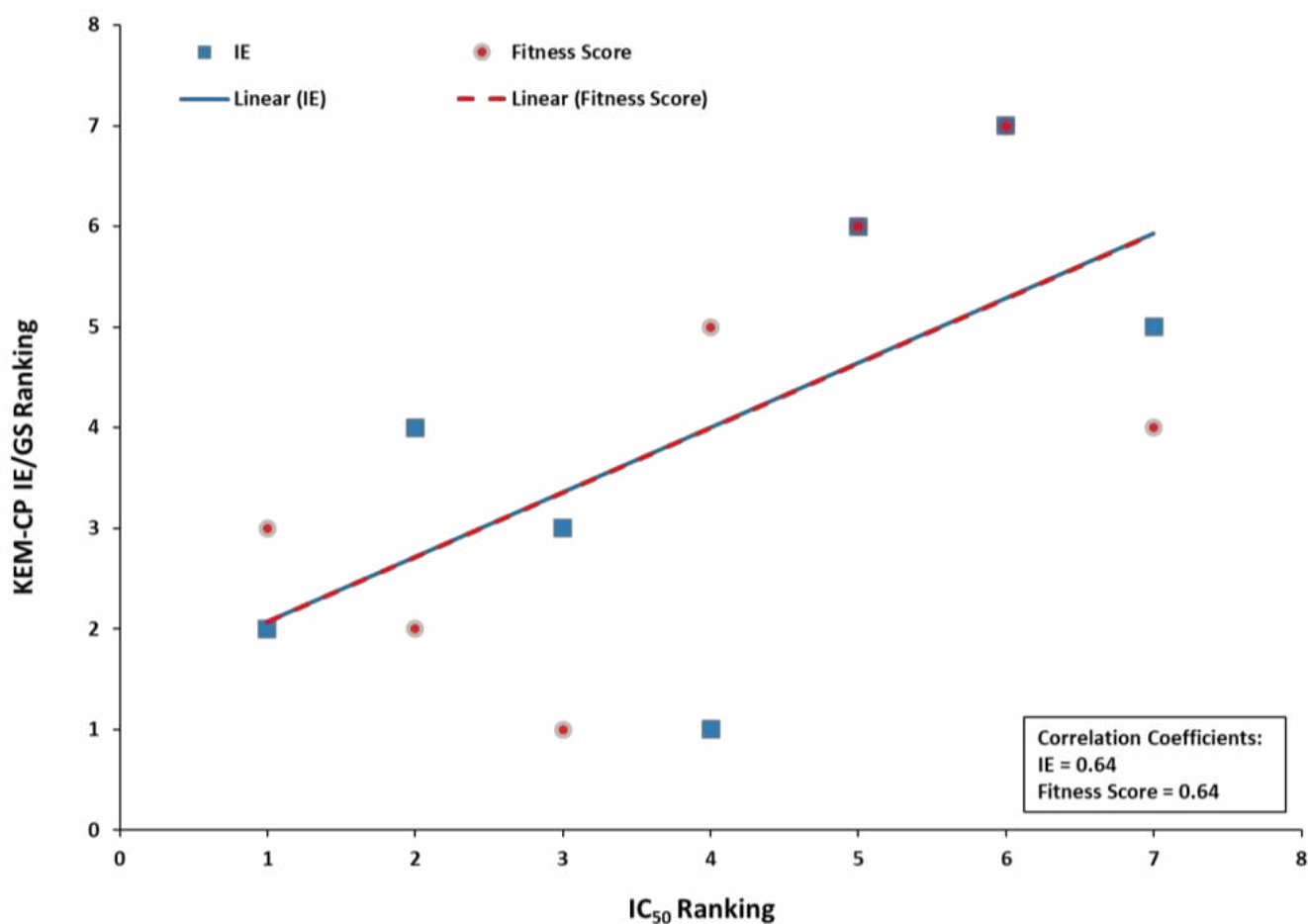
Figure 4. Plot showing IC 50 ranking distribution with the KEM-CP IE and GoldScore fitness score rankings for the best predicted poses as listed in Table S15, Supplementary Materials.
