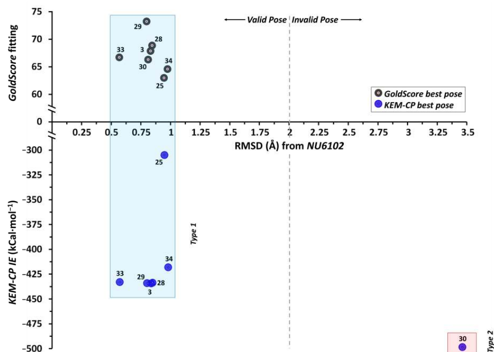
Figure 3. Distribution of RMSD ( \text{\AA} ) vs. fitting score from GoldScore and vs. KEM-CP based average IE of CDK2 ligands as listed in Tables 4 and 5.
