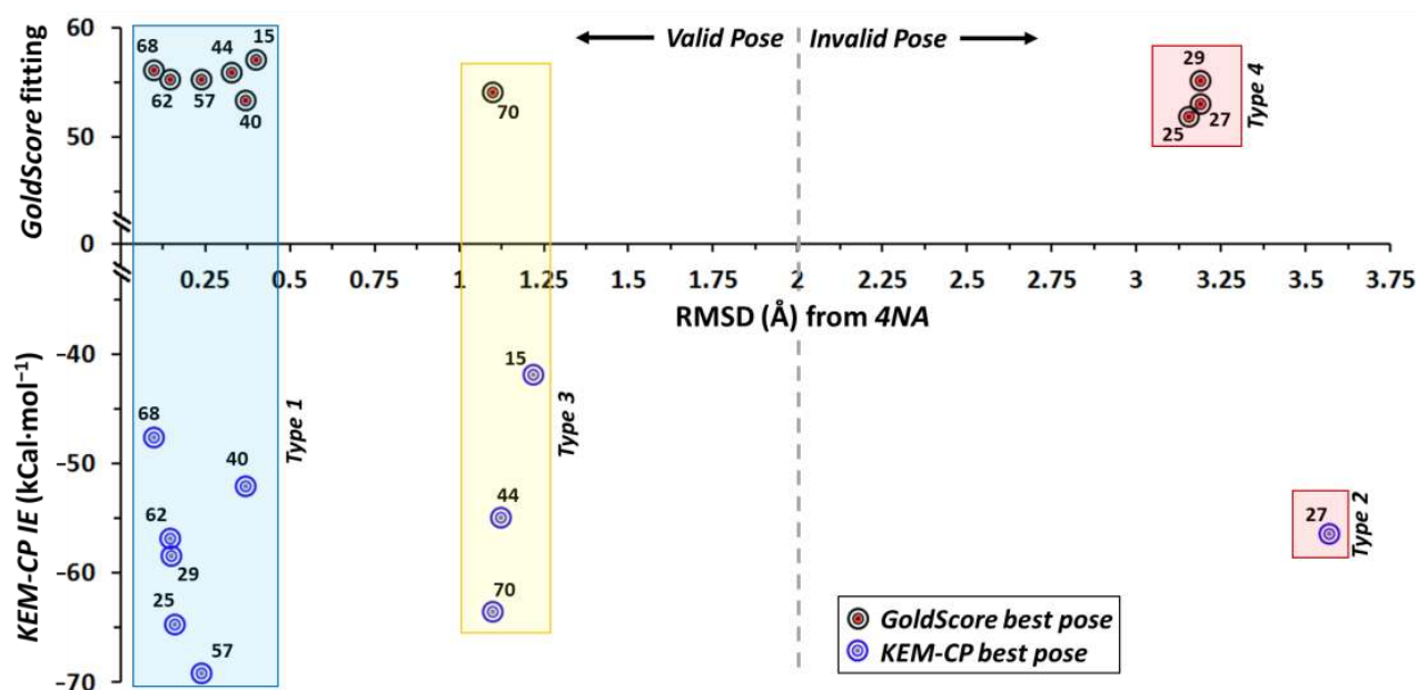
Figure 5. Distribution of RMSD (Å) vs. fitting score from GoldScore and vs. KEM-CP based average IE of ER \beta ligands as listed in Tables 6 and 7.
