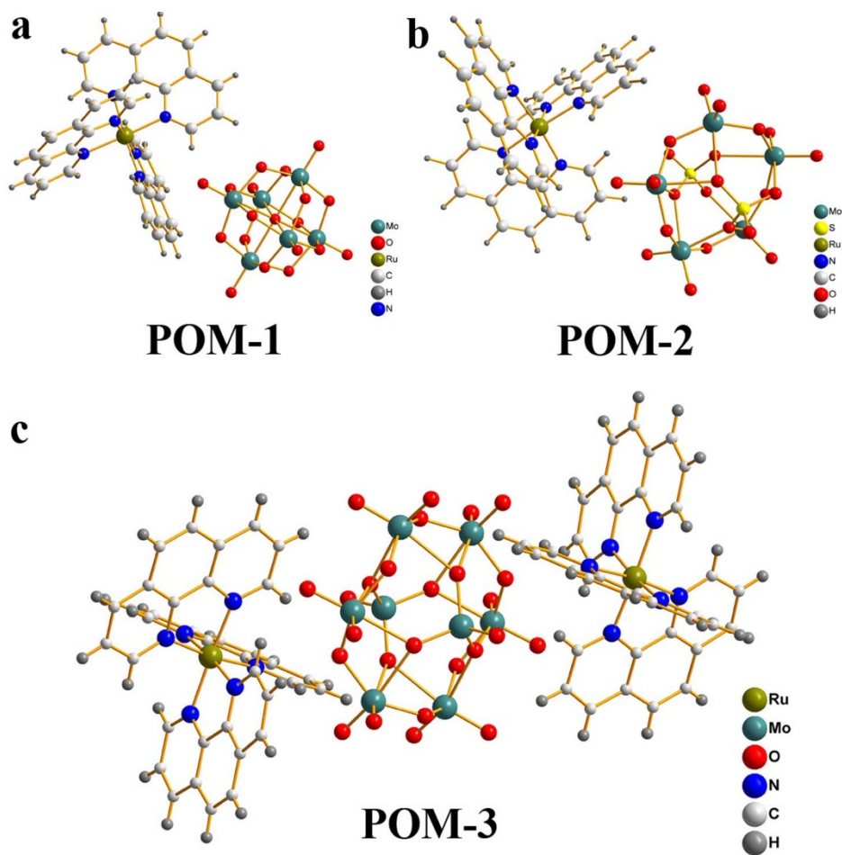
Figure 1 | The structures of hybrid materials POM-1–3.
