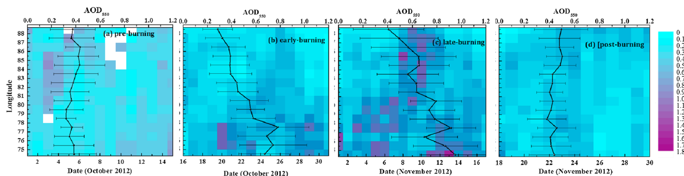
Figure 4. Longitudinal variation of the AOD 550nm via Terra MODIS observations over IGP region during the four subperiods of the postmonsoon season 2012. The line expresses the averaged longitudinal variation during each period. The vertical bars express one standard deviation from the mean latitudinal-averaged value at each longitude. The area that has been used for the analysis is 22.5°–31.5°N, 74.5°–88.5°E, excluding the pixels over Himalayan range and Tibetan Plateau. White pixels correspond to lack of data.
