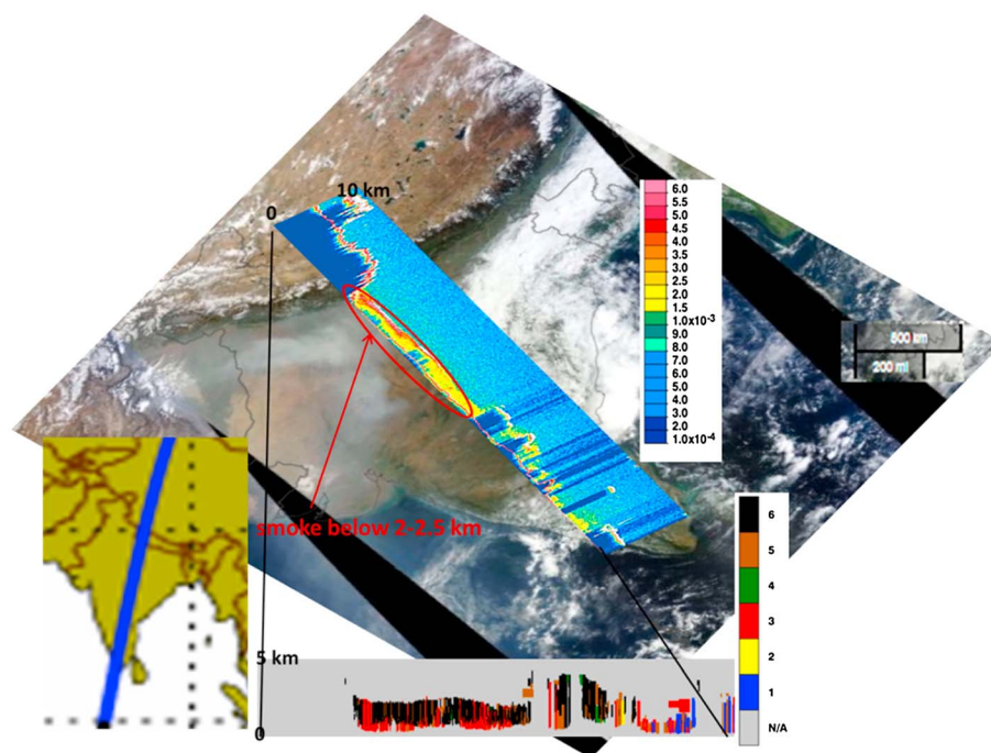
Figure 5. Total attenuated backscatter ( \text{km}^{-1} \text{sr}^{-1} ) at 532 nm from nighttime CALIPSO observations on 5 November 2012 (20:31–20:44 UTC, +5:30 LST). The background image corresponds to Terra MODIS on 5 November 2012. The CALIPSO trajectory over India is shown in the inset image, as well as the aerosol subtype (1: clean marine, 2: dust, 3: polluted continental, 4: clean continental, 5: polluted dust, and 6: smoke).
