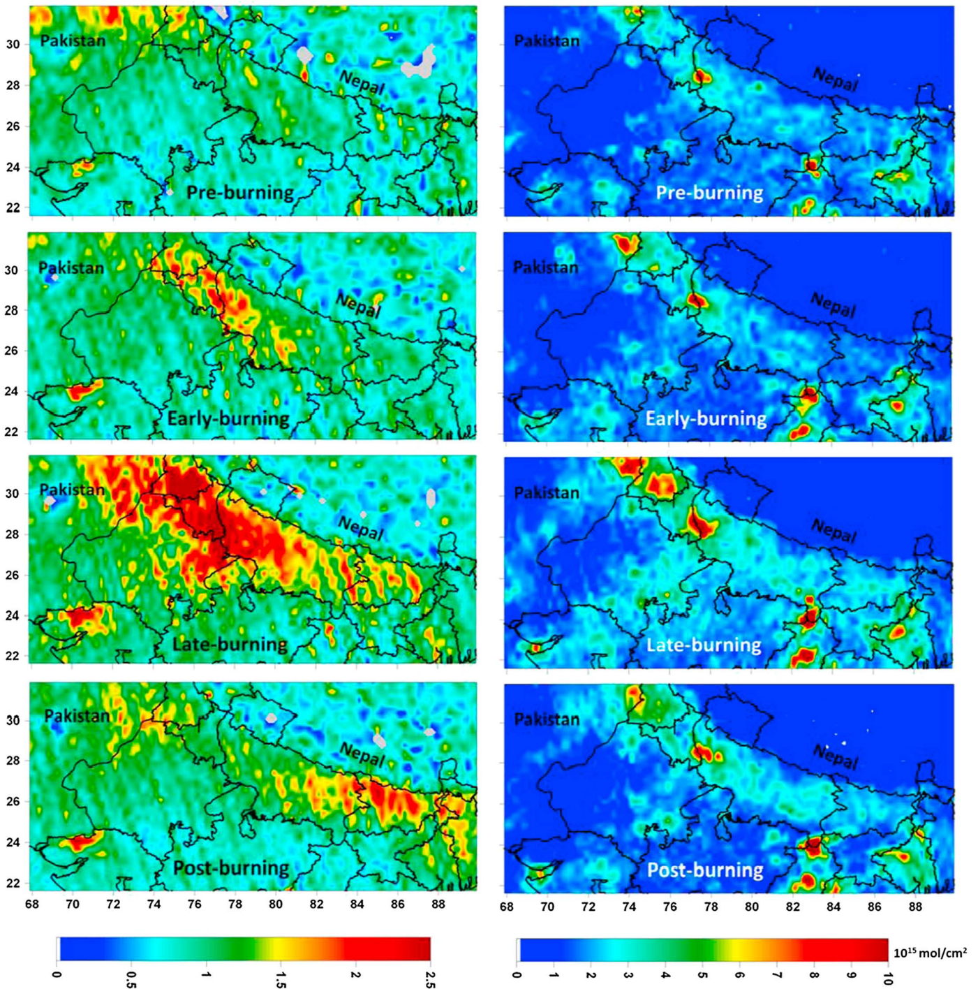
Figure 3. Spatial distribution of (left) Aura OMI-AI and (right) tropospheric \text{NO}_2 concentrations over IGP during the four subperiods of the postmonsoon season 2012.
