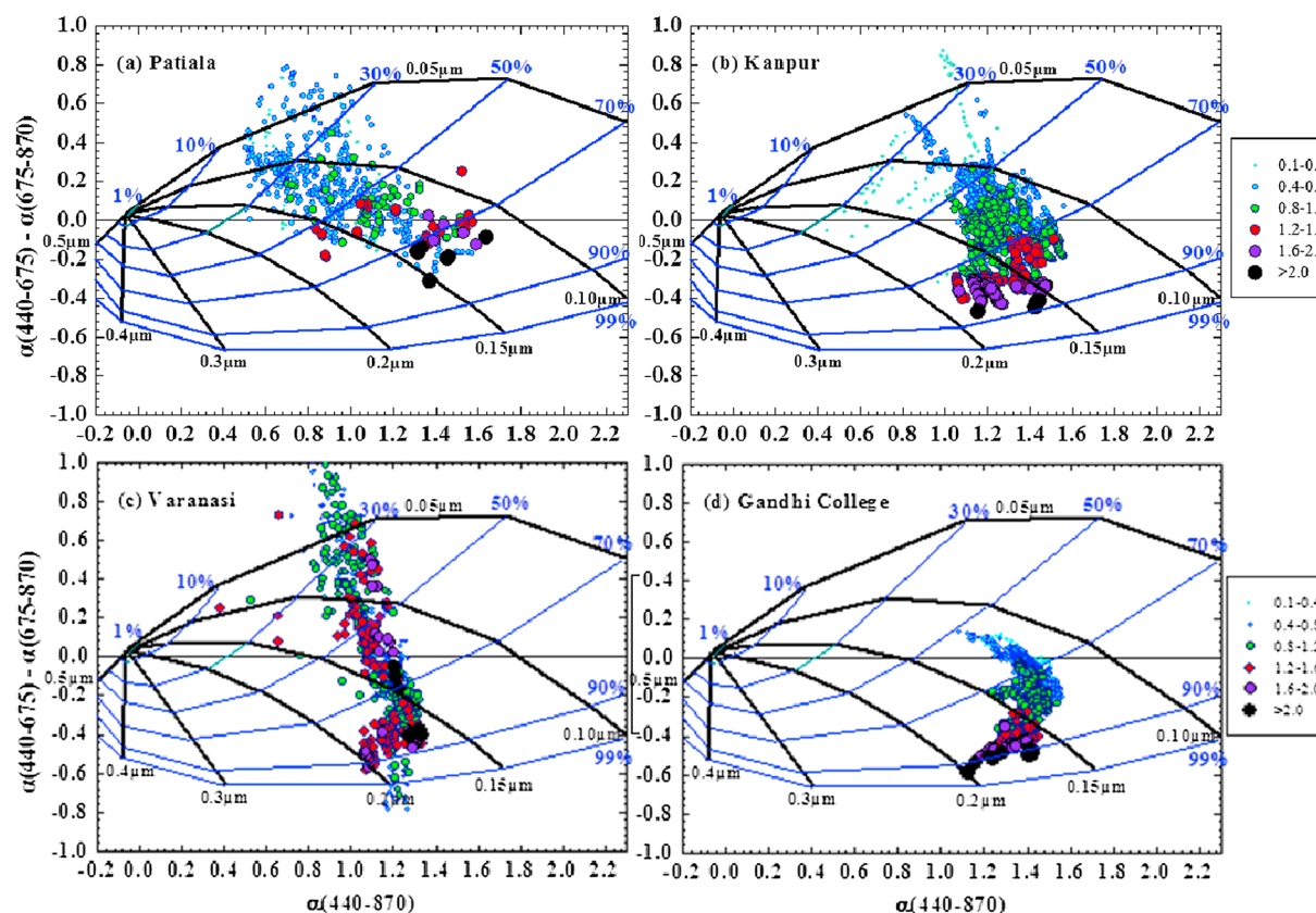
Figure 15. Ångström exponent difference \Delta\alpha = \alpha(440-675) - \alpha(675-870) as a function of the \alpha_{440-870} and AOD_{500\text{ nm}} (color-sized scale) over four IGP sites during postmonsoon 2012, for bimodal lognormal size distribution. The black lines indicate the fixed effective radius ( R_f ) of the fine mode and the blue lines the fixed fraction ( \eta ) of fine mode to the AOD.
