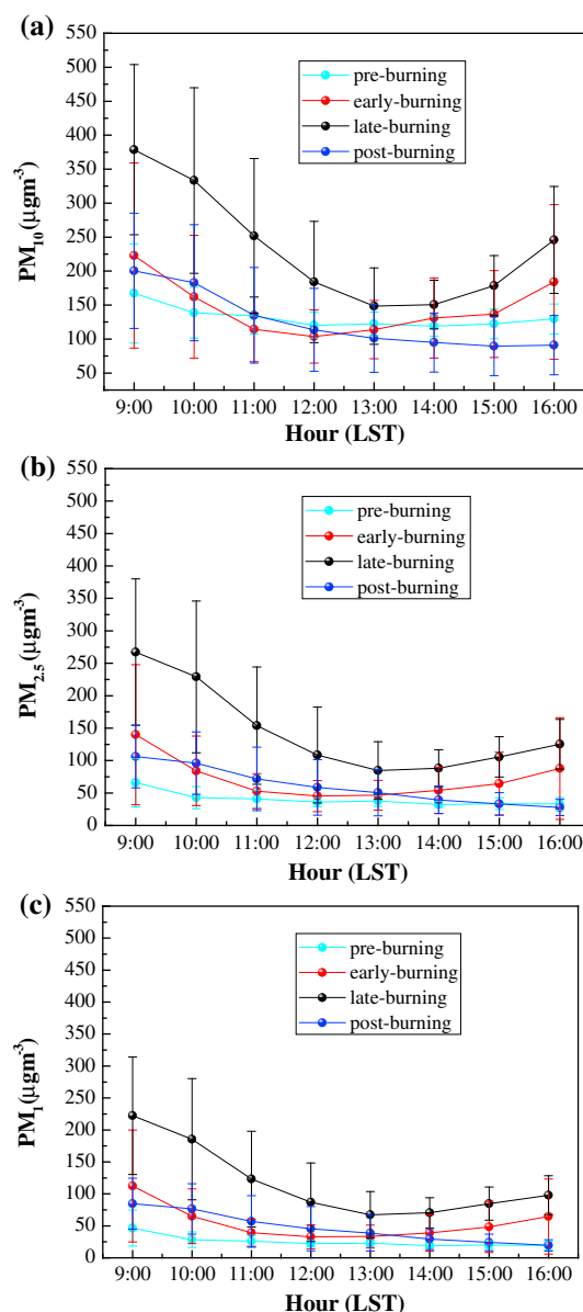
Figure 9. Mean semidiurnal (09:00–16:00 LST) variation of the (a) \text{PM}_{10} , (b) \text{PM}_{2.5} , and (c) \text{PM}_1 concentrations at Patiala during the four subperiods of the postmonsoon 2012. The vertical bars correspond to 1 standard deviation of the mean.
