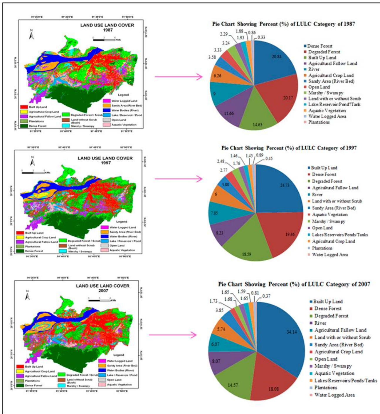
Figure 4. Allocation of LULC and percent (%) of LULC of 1987, 1997 and 2007 [9].
