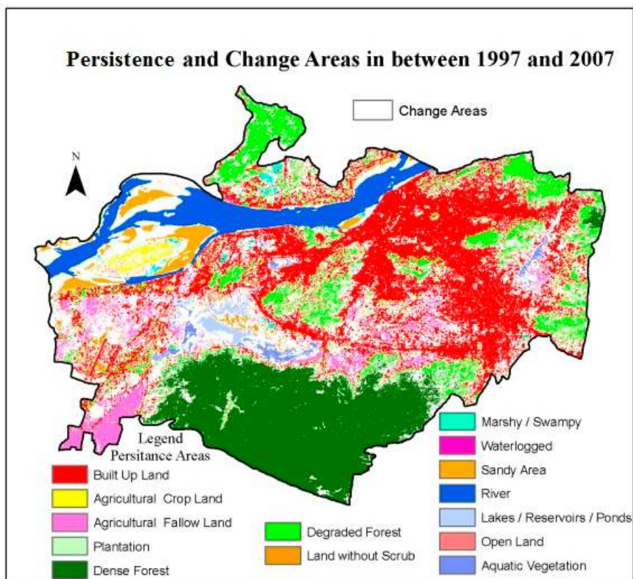
Figure 10. Persistence and change areas between 1997 and 2007.
