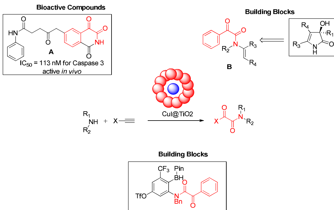
Scheme 1. Catalyst comprising of TiO 2 encapsulated CuI nanoparticles (CuI@TiO 2 ) for the synthesis of ketoaryl amides (from alkynes) and their representative molecules as building blocks and bioactive compounds
