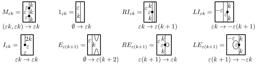
FIGURE 2.1. Generating tangles.
