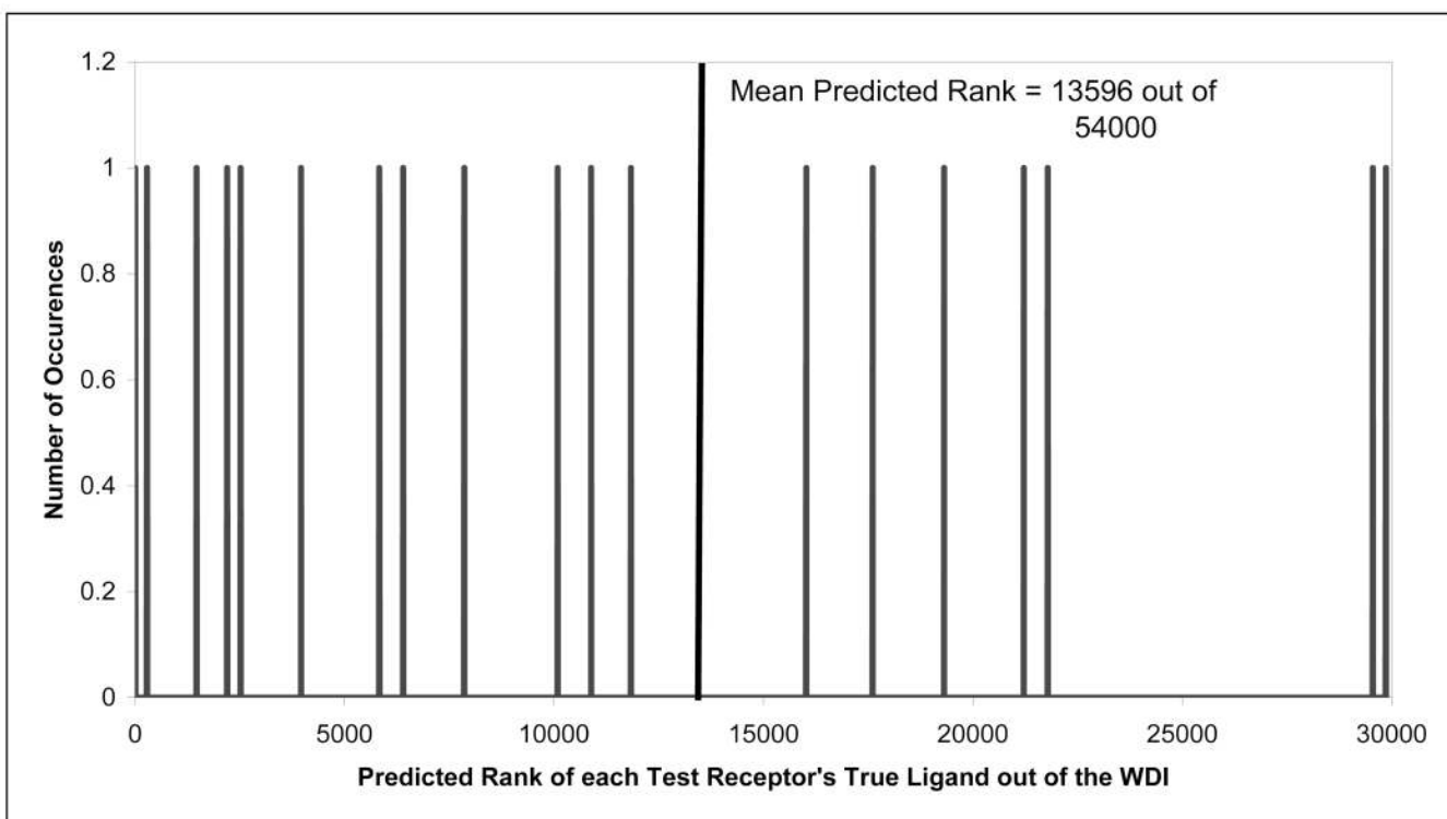
Figure 7. Predictive ability of CoLiBRI to identify ligands of 22 test binding pockets from the WDI when there are no receptors of the same family in the training set.
