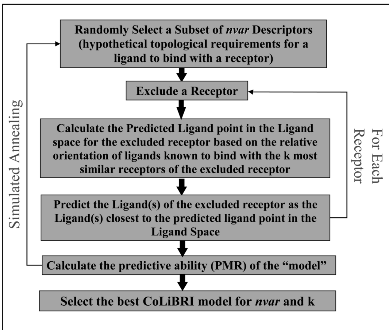
Figure 3. Flowchart of CoLiBRI Method
