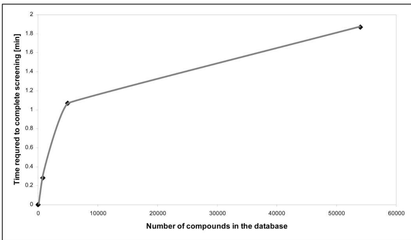
Figure 8. Time required for 100 CoLiBRI models to screen a single test receptor against various compound libraries on a P4 machine using a max. limit of 5,000 sorted hits displayed as output.
