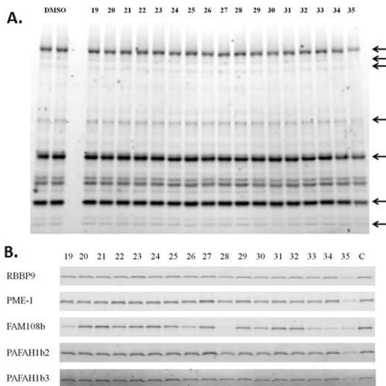
Fig. 5. Inhibition of SHs by 1,3,4-oxadiazol-2-ones. A. ABPP Gel-based inhibition assay of compounds 19-35 using a HeLa cell lysate. The lysate (1mg/mL total protein) was incubated with 100 \mu M of each compound ( 19-35 ) for 30 minutes. Rhodamine fluorophosphonate (FP-Rh) (100 nM) was then added and the reaction mixture was incubated for 10 minutes before being quenched with a denaturing buffer. The samples were subjected to SDS-PAGE and the rhodamine-labeled protein bands were visualized using a Typhoon gel scanner. B. A similar experiment as in part A was conducted except that five purified, recombinant SH enzymes (2 \mu M each) were employed in place of the cell lysate. In this case the compounds were employed at a concentration of 200 \mu M.
